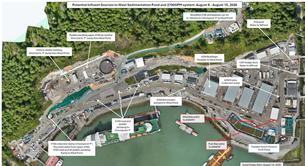
Figure 3: West Catchment contact water management facilities (August 9 – 15).
