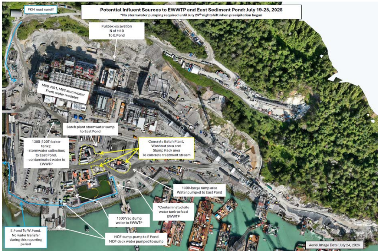
Figure 2: East Catchment contact water management facilities (July 19 - 25).
