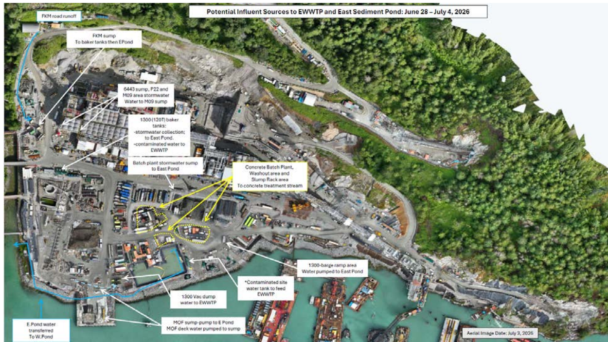
Figure 2: East Catchment contact water management facilities (June 28 – July 4).
