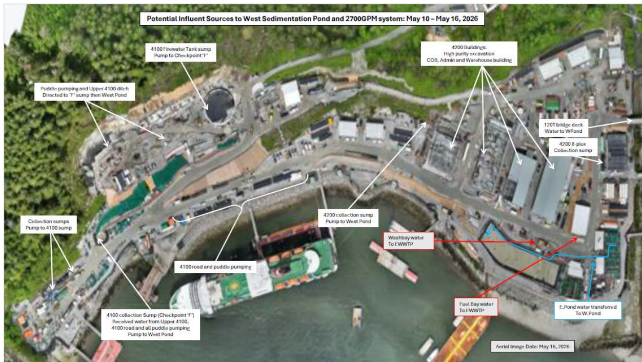
Figure 3: West Catchment contact water management facilities (May 10 – 16).
