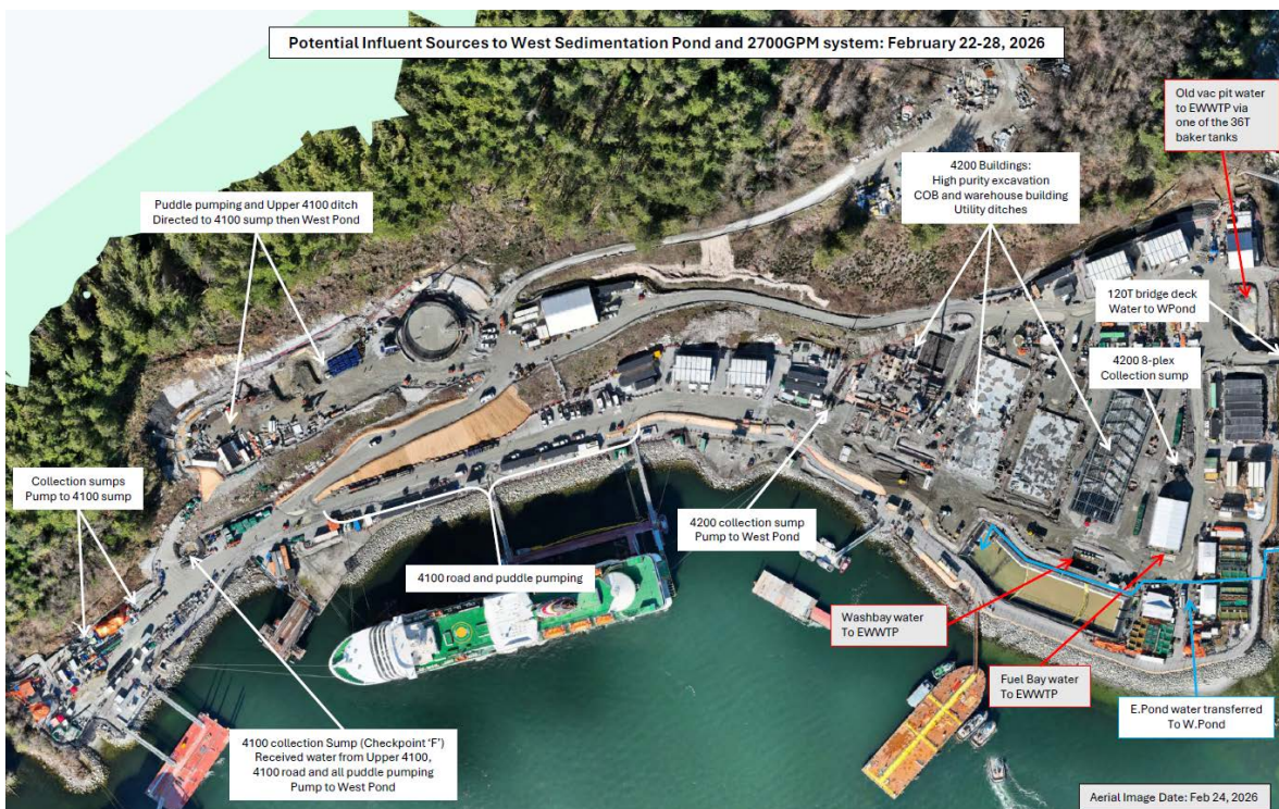
Figure 3: West Catchment contact water management facilities (February 22 – 28).
