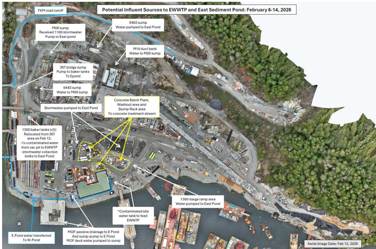
Figure 2: East Catchment contact water management facilities (February 8 – 14).
